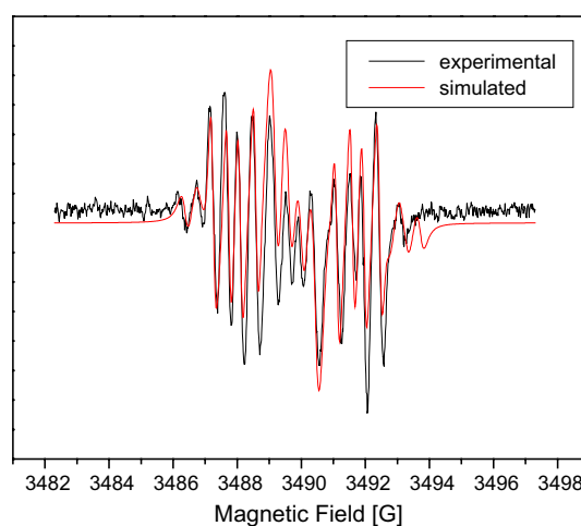
Figure 3. Experimental and simulated spectra of 4c 1 radical species.
