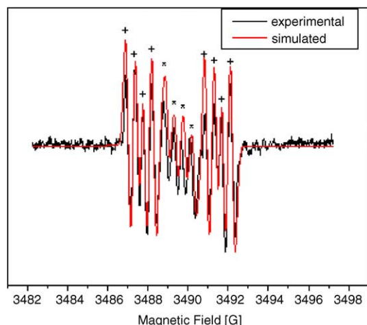
Figure 4. Experimental and simulated spectra of mixture of 4c 2 (+) and 4c 3 (*) radical species.
