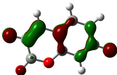
Figure 6. SOMO of radical 4c 1 .
