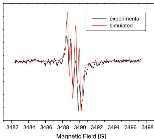
Figure 5. Experimental and simulated spectra of 4c 3 radical species.
